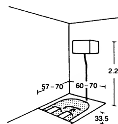
⑧ Squatting WC (French style)
